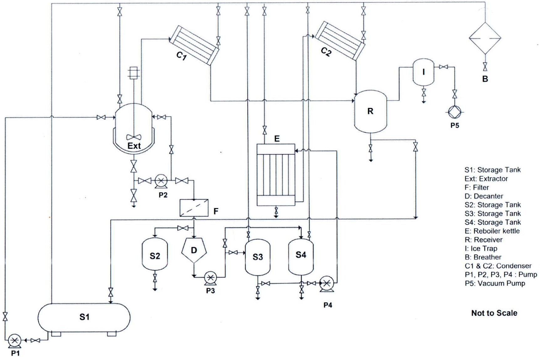
Flow Chart for Solvent Extraction Plant
